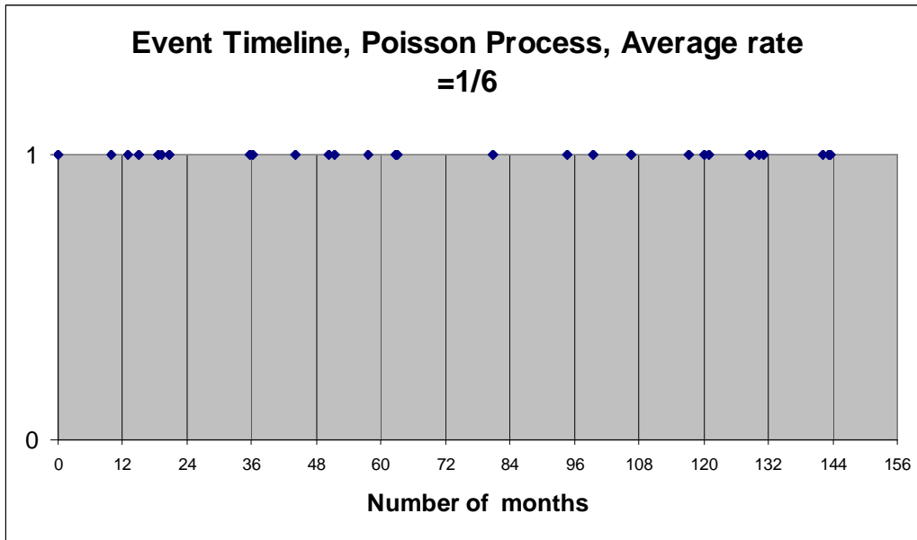
FIGURE 3—Example of a 28 Event Time Sequence for a Poisson Process with Average Time Between Events of 6 Months
