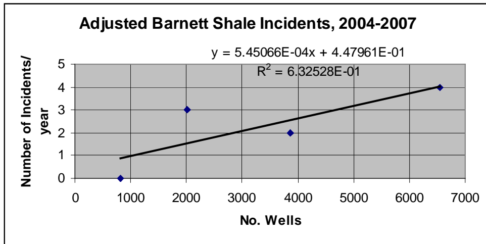
FIGURE 2—Number of Gas Gathering Line Incidents per Year vs Estimated Number of Operational Wells in the Barnett Shale
